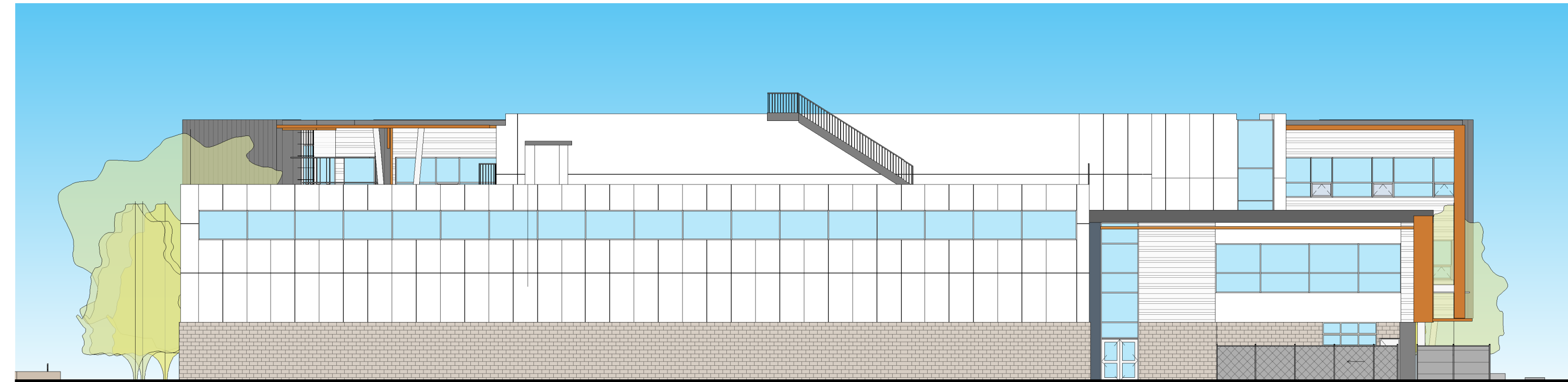
EAST ELEVATION 1 : 200
